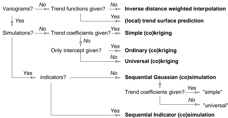
Figure 2: Prediction method decision tree of predict.gstat (or krige ); each of the prediction methods may apply to points, rectangular blocks, or irregular blocks, and may use all data or a selection of local data in a local neighbourhood around each prediction location
