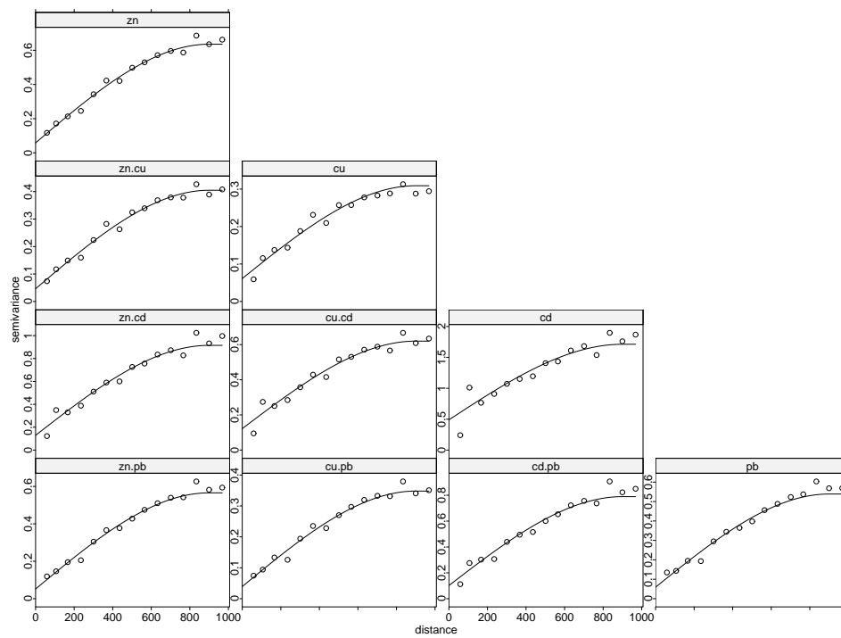
Figure 1: direct sample variograms (diagonal), cross variograms (off-diagonal) and fitted linear model of coregionalisation for the four heavy metal variables in the meuse data set
