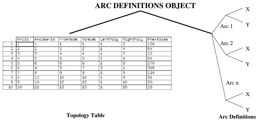
Figure 2: Structure of an arc definitions (from file arc.adf ) imported in R. Lines represent lists, while X and Y are both vectors of coordinates.
