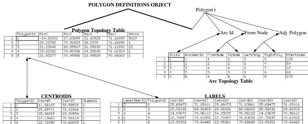
Figure 3: Relationships between arcs, polygons, centroids and labels. Notice that values of From Node and Adjacent polygon depend on the way we move along the arcs.
