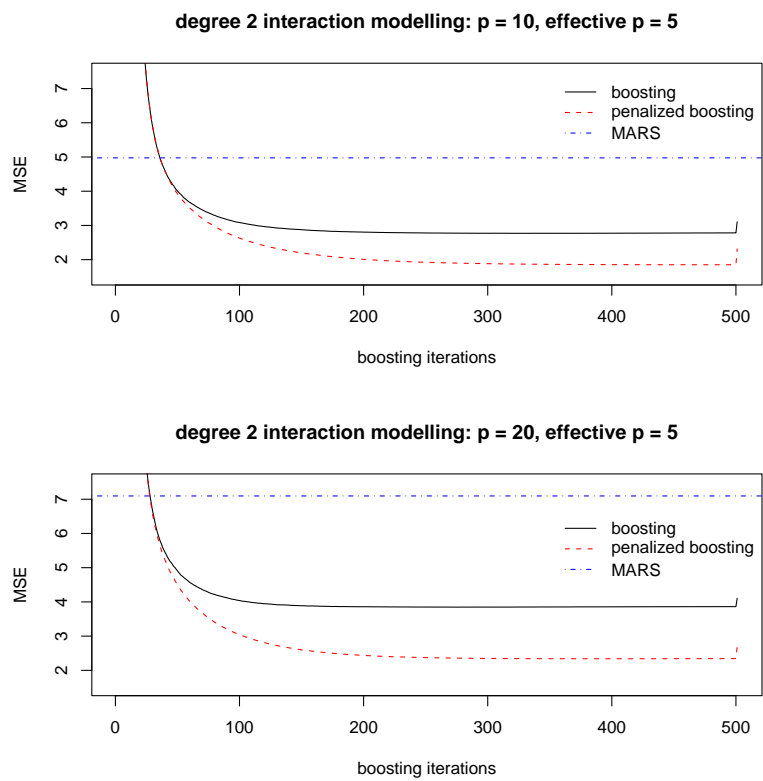
Figure 1: Mean squared error for L_2 Boosting using componentwise thin plate splines, a penalized version of L_2 Boosting, and MARS in the Friedman #1 model (6) with sample size n = 50 . Top: p = 10 . Bottom: p = 20 . The performance with AIC-stopped boosting iterations is indicated at abscissa x = 501 .
